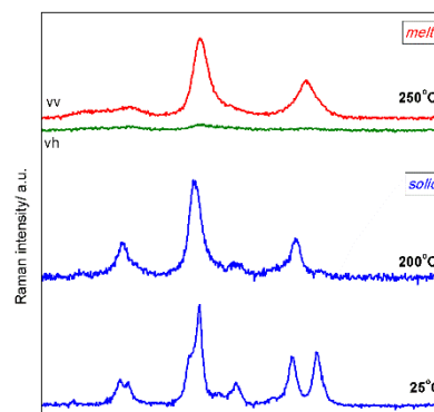
Fig 1. Raman spectra....
